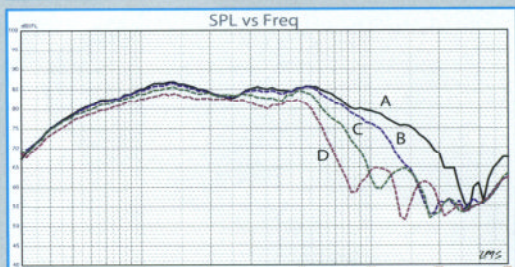
FIGURE 11: EM 1308 horizontal on- and off-axis frequency response (A = 0°; B = 15°; C = 30°; D = 45°).
