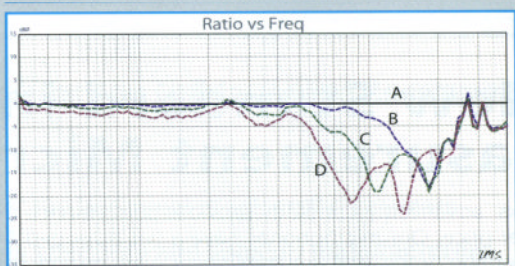
FIGURE 12: EM 1308 normalized on- and off-axis frequency response (A = 0°; B = 15°; C = 30°; D = 45°).
