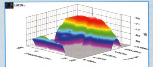
FIGURE 15: EM 1308 SoundCheck STFT surface intensity plot.
