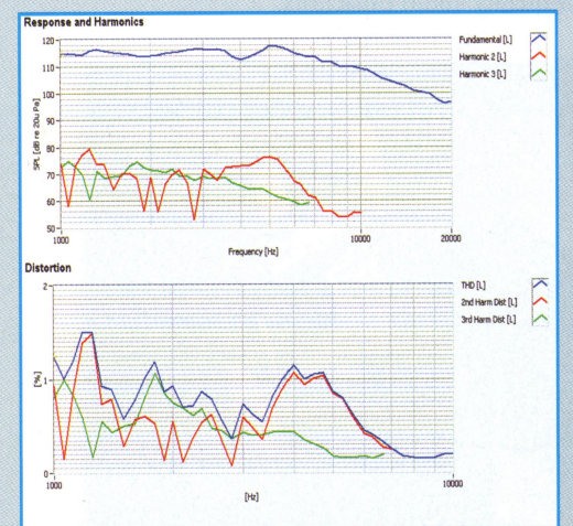
FIGURE 16: Morel EM 1308 SoundCheck distortion plots.
