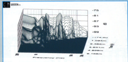
FIGURE 14: EM 1308 SoundCheck CSD waterfall plot.
